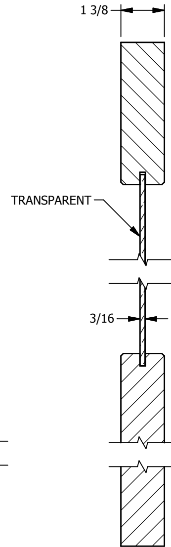
SECTION A-A PMT
