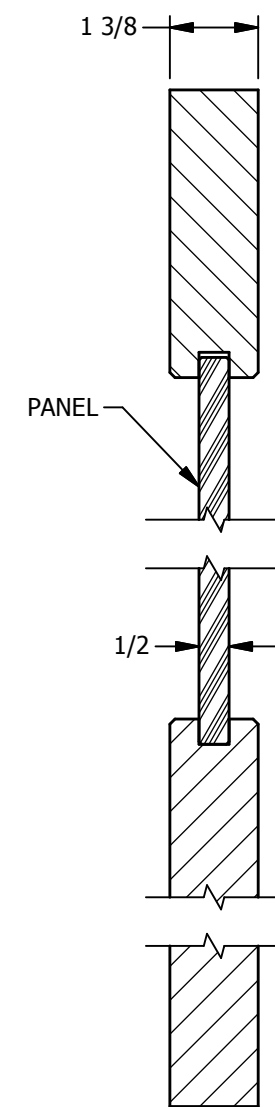
SECTION A-A PMP
