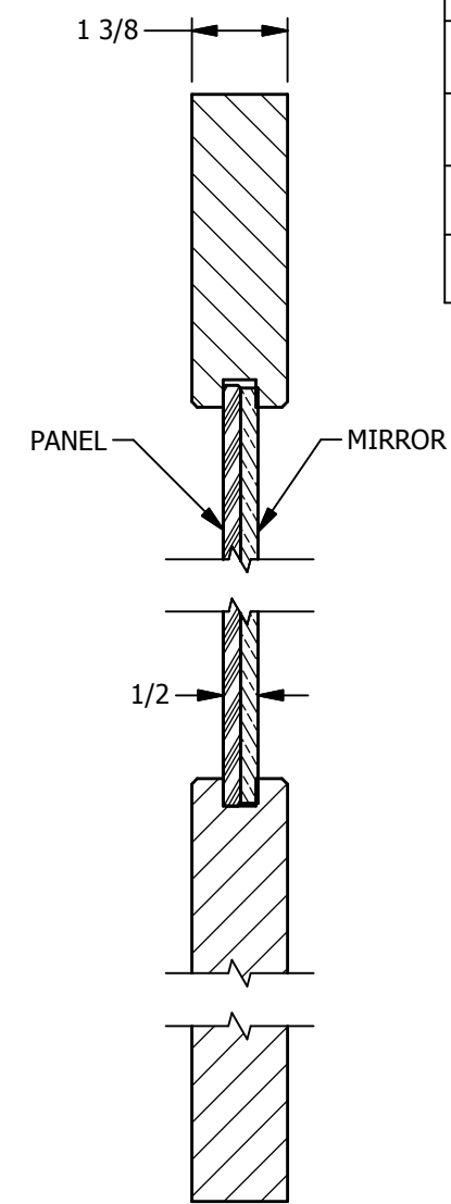
SECTION A-A PMM
